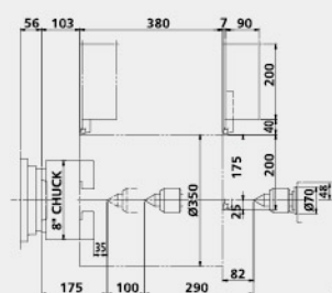
FTC-350 Working Range
