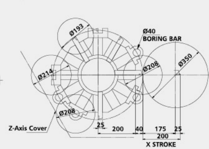
8-Position Turret Tool Interference Diagram (STD)
