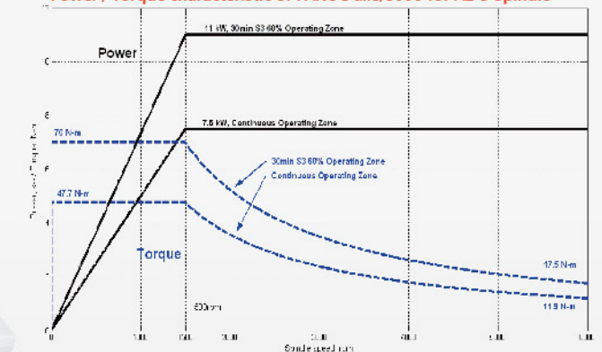
Power / Torque characteristic of FANUC oil8/8000 for A2-5 Spindle
