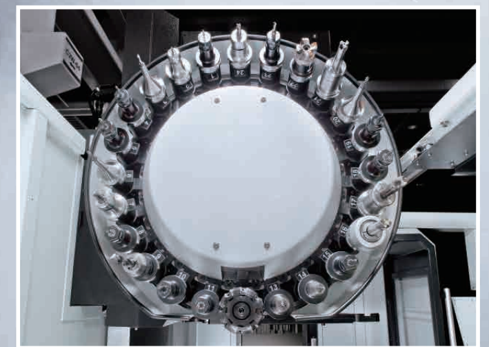
24T Disc type tool magazine
